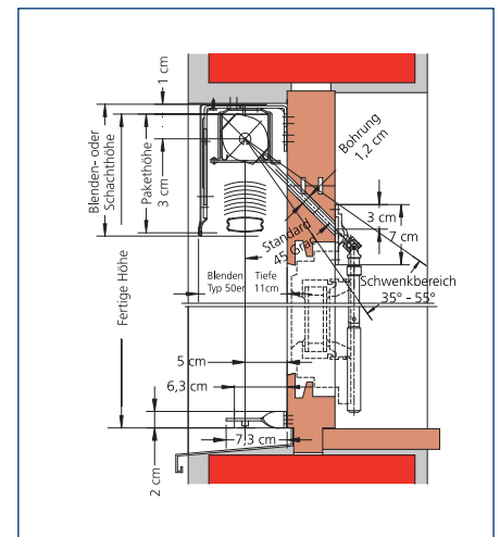
Typ Ambassador AA50
